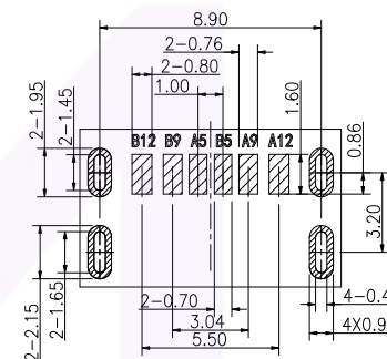
RECOMMENDED PCB LAYOUT (TOLERANCE: ±0.05)
