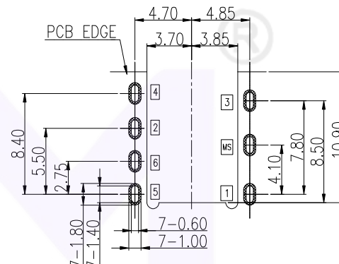
RECOMMENDED P.C.B LAYOUT(t=1.0mm) TOP VIEW (TOLRANCE:±0.05)
