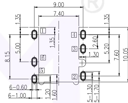
TOP VIEW (TOLRANCE:±0.05)
