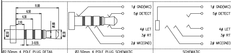
02.50mm 4 POLE PLUG DETAIL 02.50mm 4 POLE PLUG SCHEMATIC SCHEMATIC
