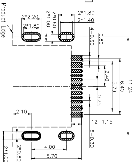
RECOMMENDED P.C.B. LAYOUT TOLERANCE UNSPECIFIED ±0.05mm
