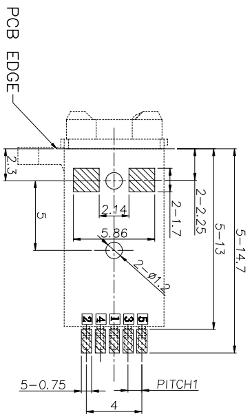
RECOMMENDED P.C.B LAYOUT TOP VIEW (TOLERANCE:±0.05)
