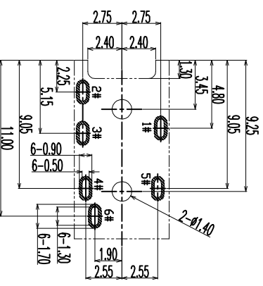
POB LAYOUT (TOP VIEW) TOLERANCE: ±0.05
